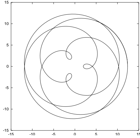
Figure 3: Epitrochoid
