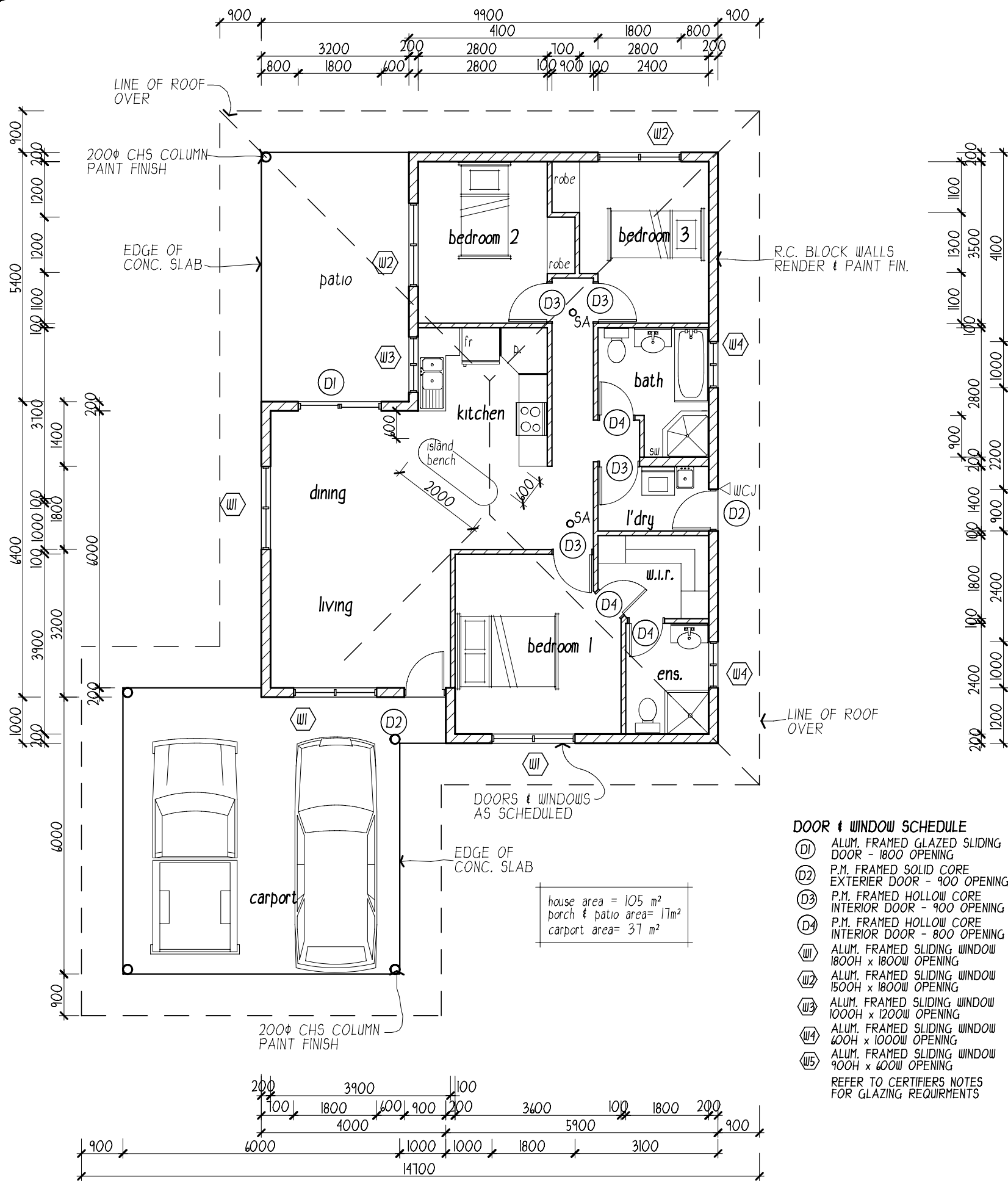
FLOOR PLAN
