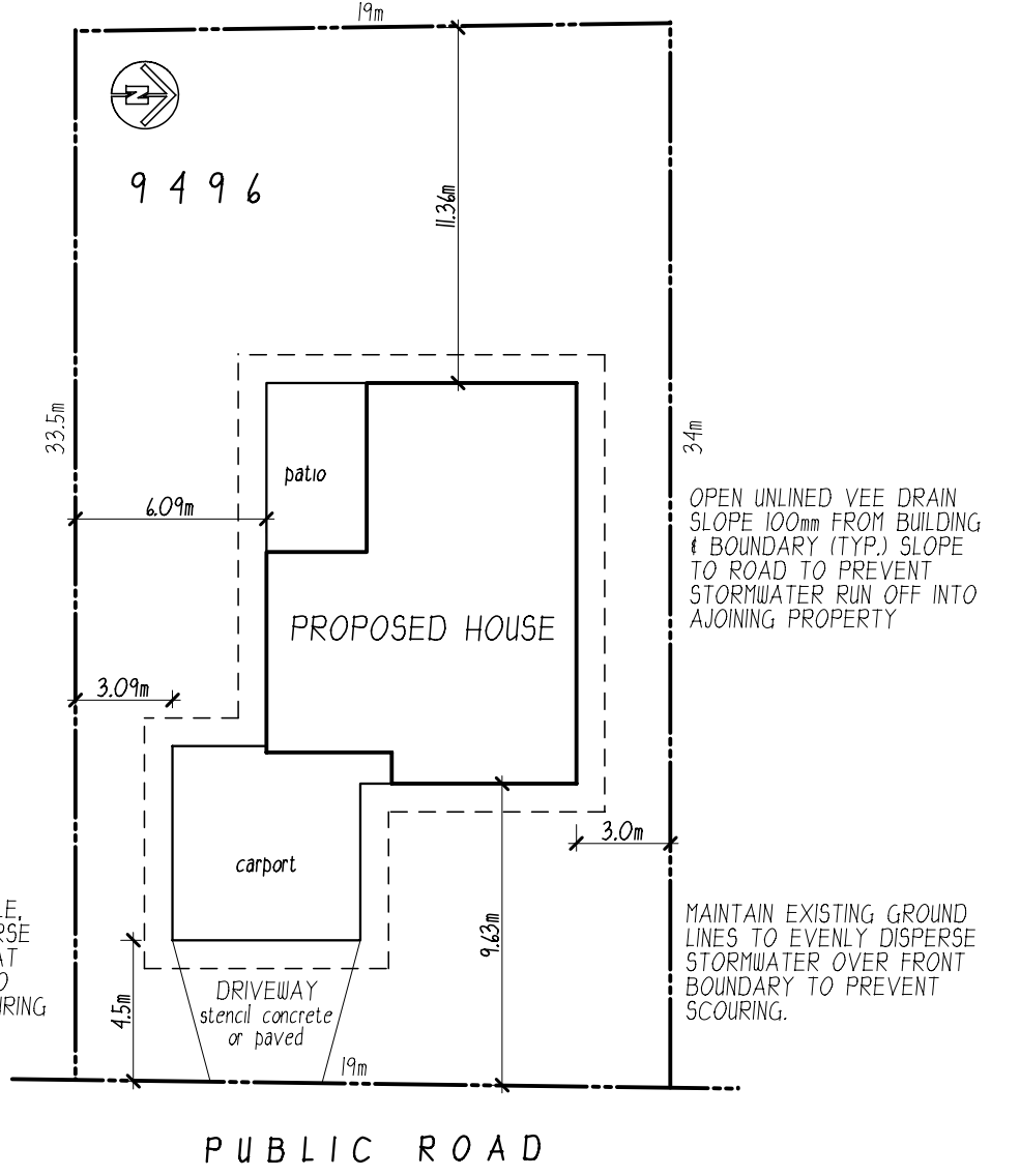
SITE PLAN
